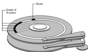
Figure 39: Clusters and sectors
