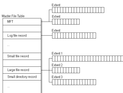
Figure 41: Simplified illustration of the MFT structure
