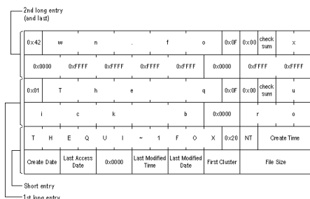
Figure 45: Example of Folder Entries for the long file name
