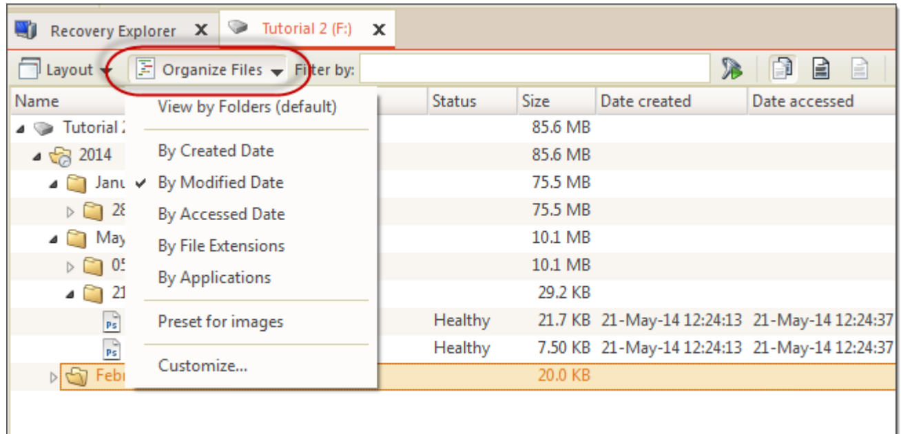
Figure 32: File Organizer menu
