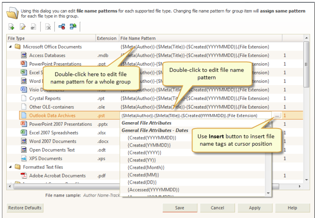
Figure 35: File Name Patterns dialog
