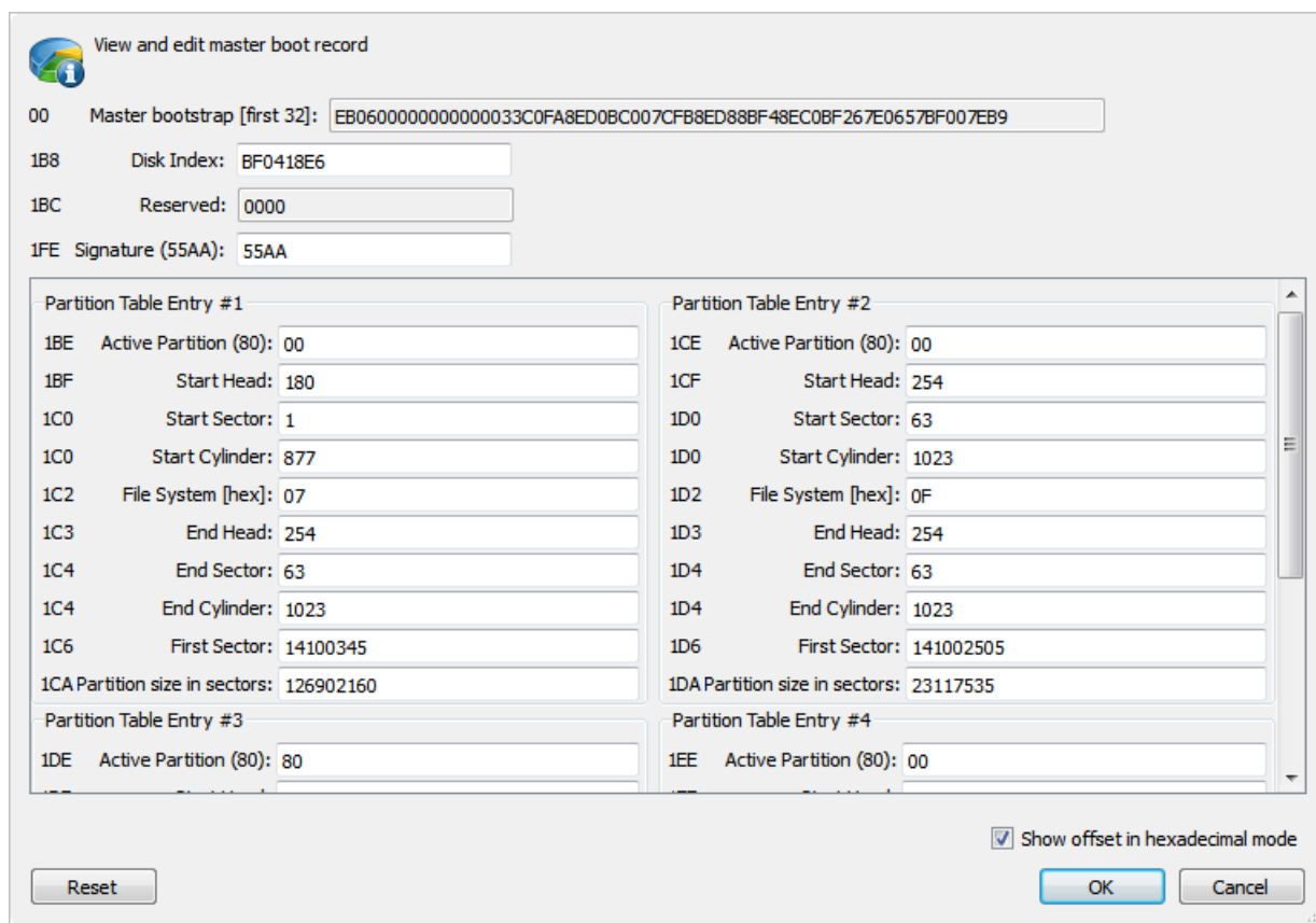
Figure 30: Edit Partition Table dialog
